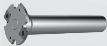
SDC 直柄小徑側銑刀 SDC INDEXABLE SIDE DISC CUTTER FOR SMALL DIAMETER
